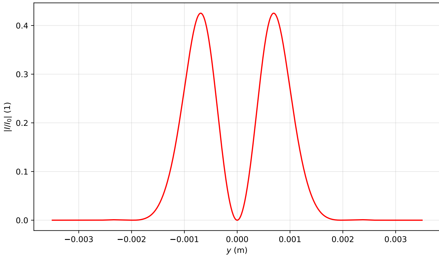
Intensity profile I(x=0, y, z=2.149)/I_0 , P_{in}=2.0P_{cr} , artificial time
